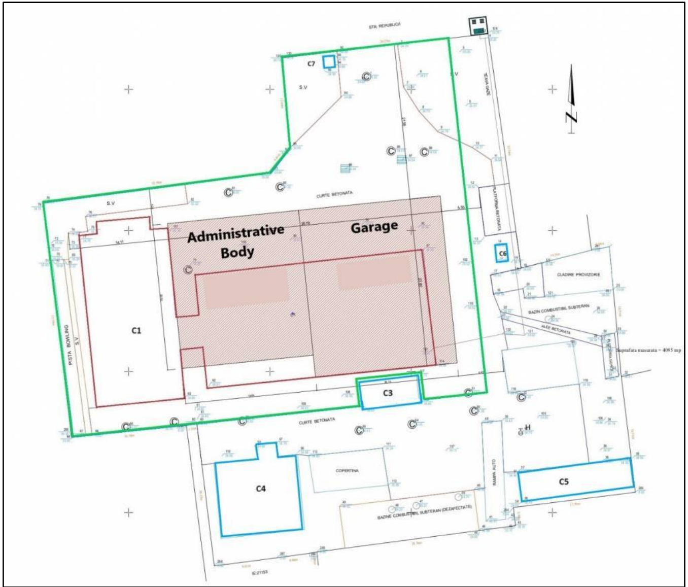
Figure 3 Proposed positioning of the new construction (sketched in orange) on the land plot. The main body C1 - marked with red - will be demolished
